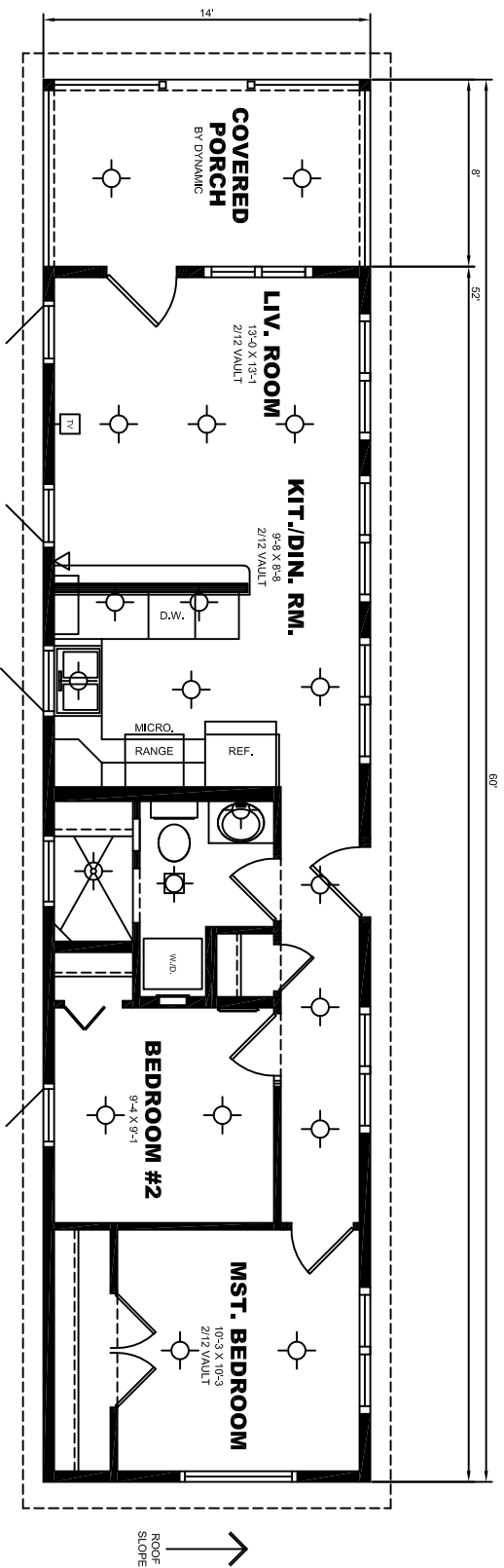
FLOOR PLAN 1/4"=1'-0" (DIMENSIONS FRAMING TO FRAMING)
