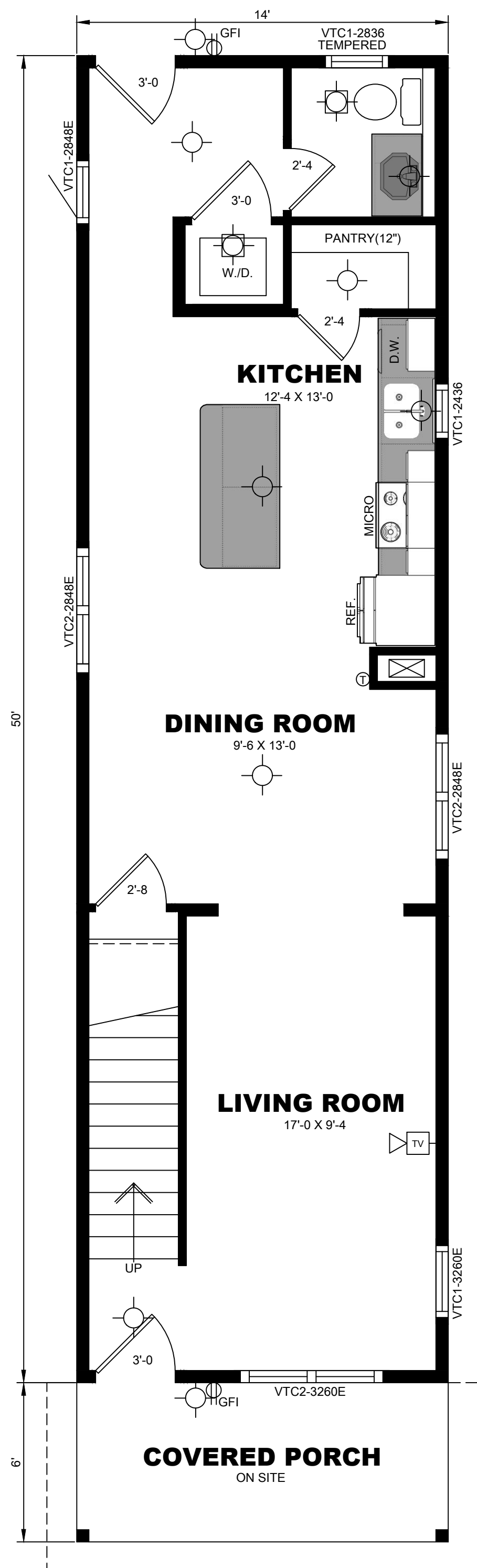
FLOOR PLAN 1/4"=1'-0" (DIMENSIONS FRAMING TO FRAMING)
