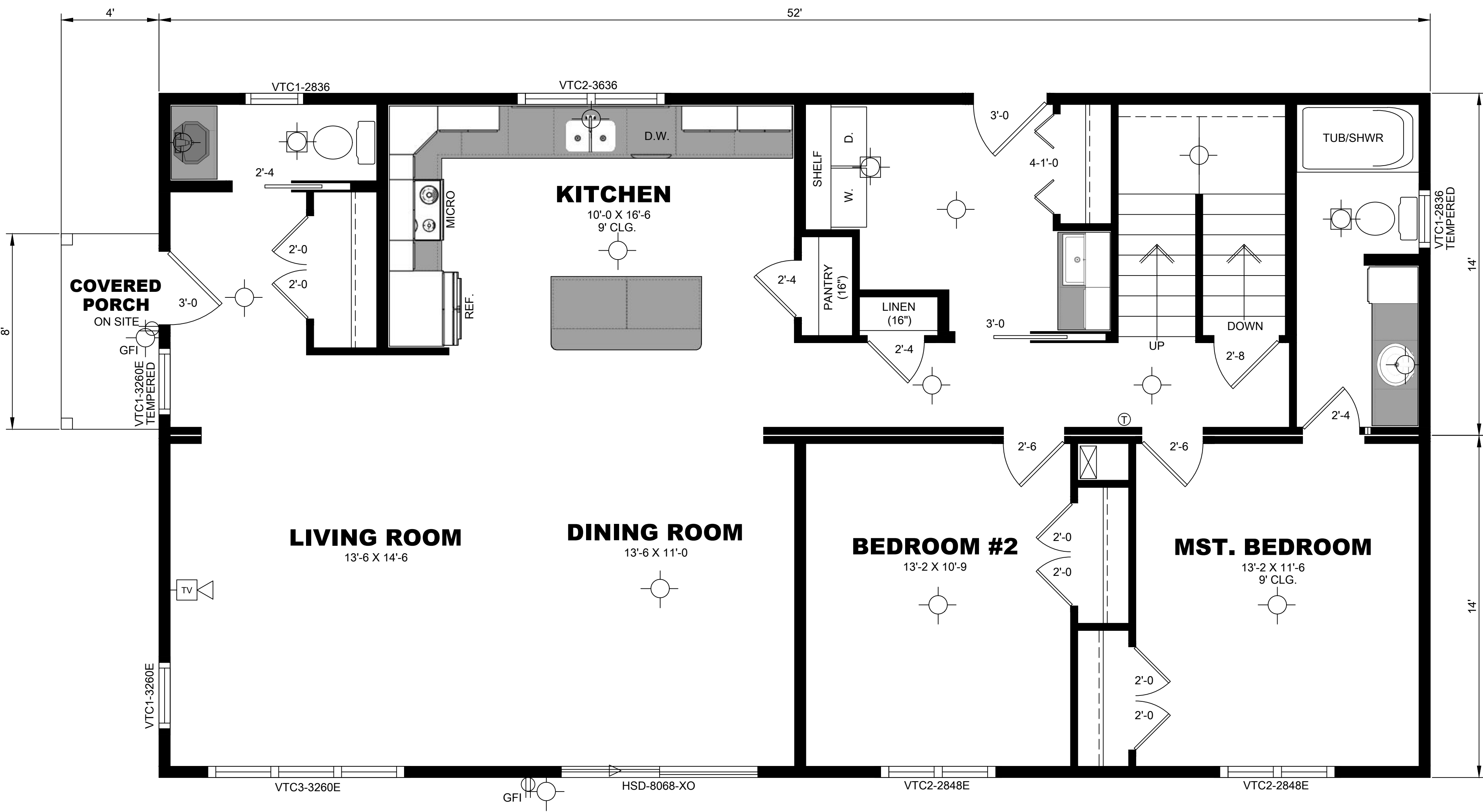
FLOOR PLAN 1/4"=1'-0" (DIMENSIONS FRAMING TO FRAMING)
