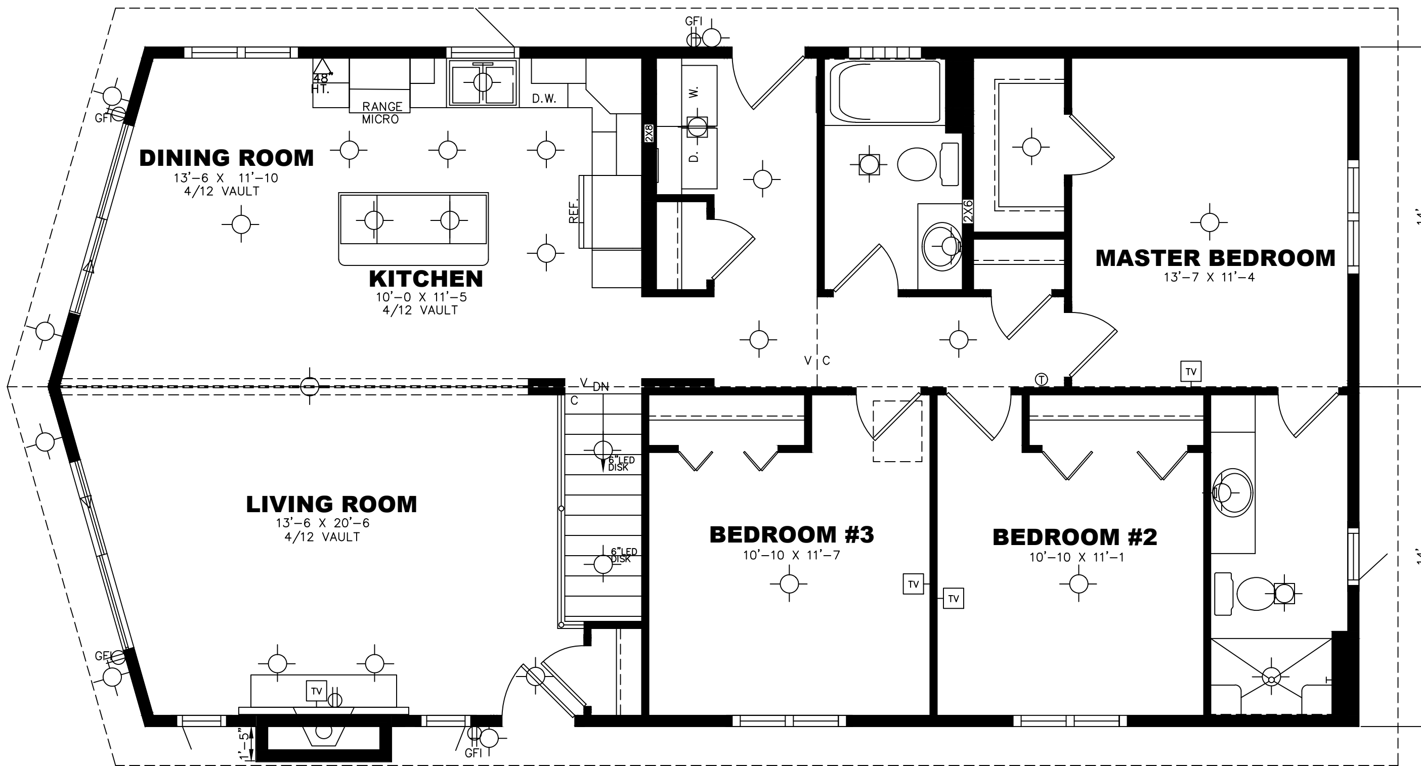
FLOOR PLAN 1/4"=1'-0" (DIMENSIONS FRAMING TO FRAMING)
