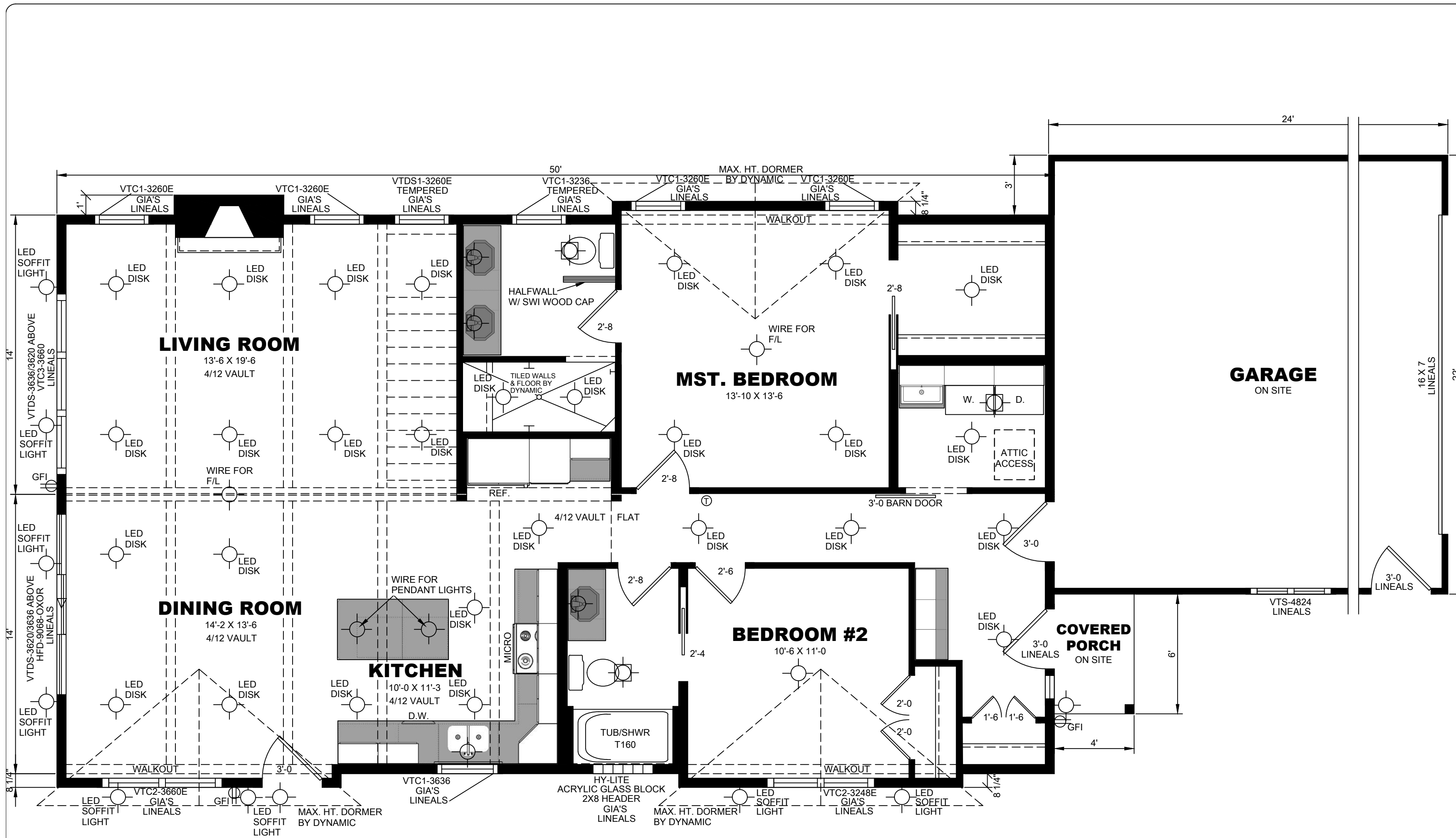
FLOOR PLAN 1/4"=1'-0" (DIMENSIONS FRAMING TO FRAMING)
