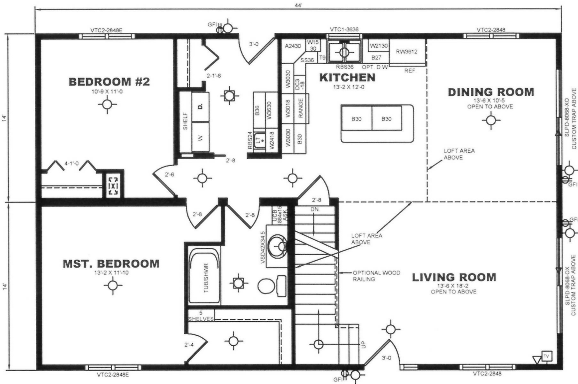
FLOOR PLAN 1/4"=1'-0" (DIMENSIONS FRAMING TO FRAMING)
