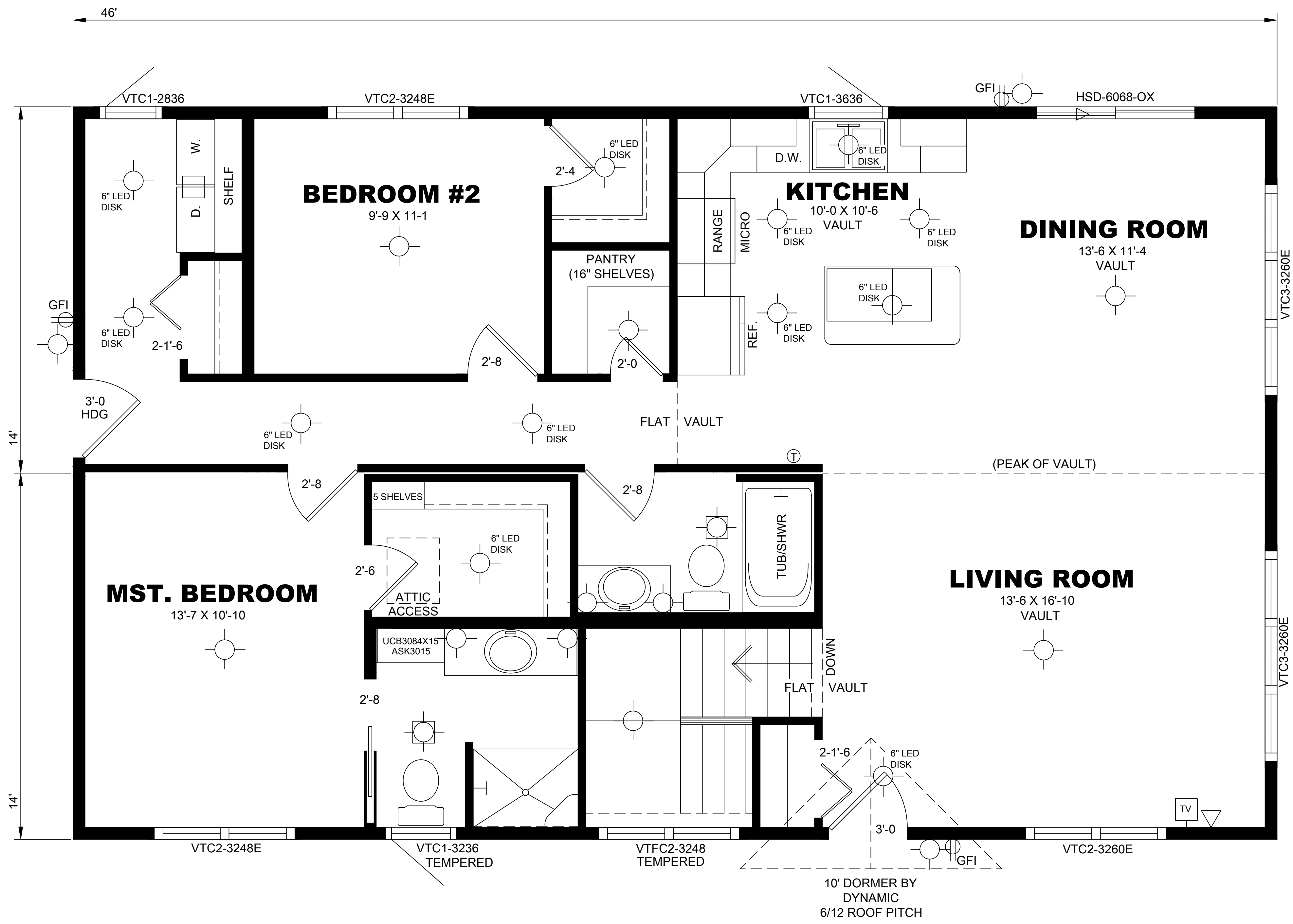
FLOOR PLAN 1/4"=1'-0" (DIMENSIONS FRAMING TO FRAMING)
