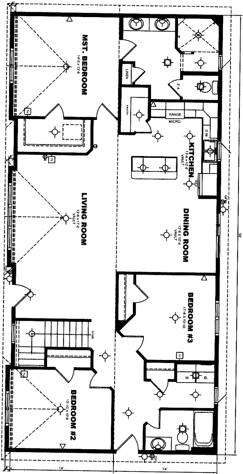
FLOOR PLAN 1/4" = 1'-0" (DIMENSIONS FRAMING TO FRAMING)
